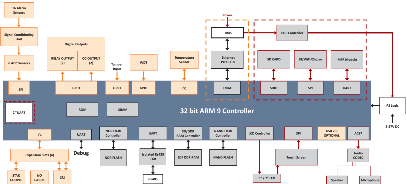
Block Diagram for Analog & Digital I/O Panel and LCD/Keypad panel Low
